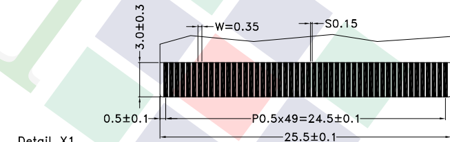
Detail X1 Scale: 4/1
